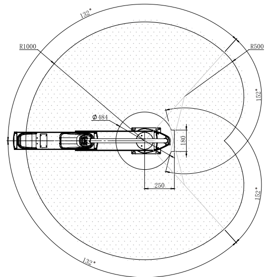
运动空间及外形安装尺寸图 Motion range and installation dimension drawing
